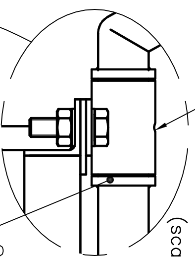
Daily greasing Detail Joint (scale 1:2)
